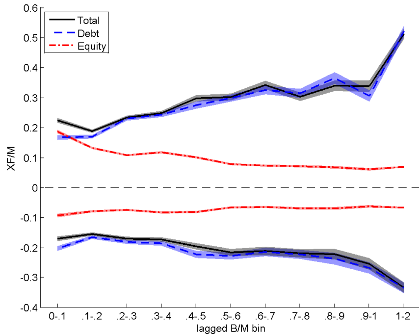
Figure 4: Empirical 5th and 95th percentiles of regression residuals \frac{XF}{M}_{it} by \frac{B}{M}_{it-1} bins
