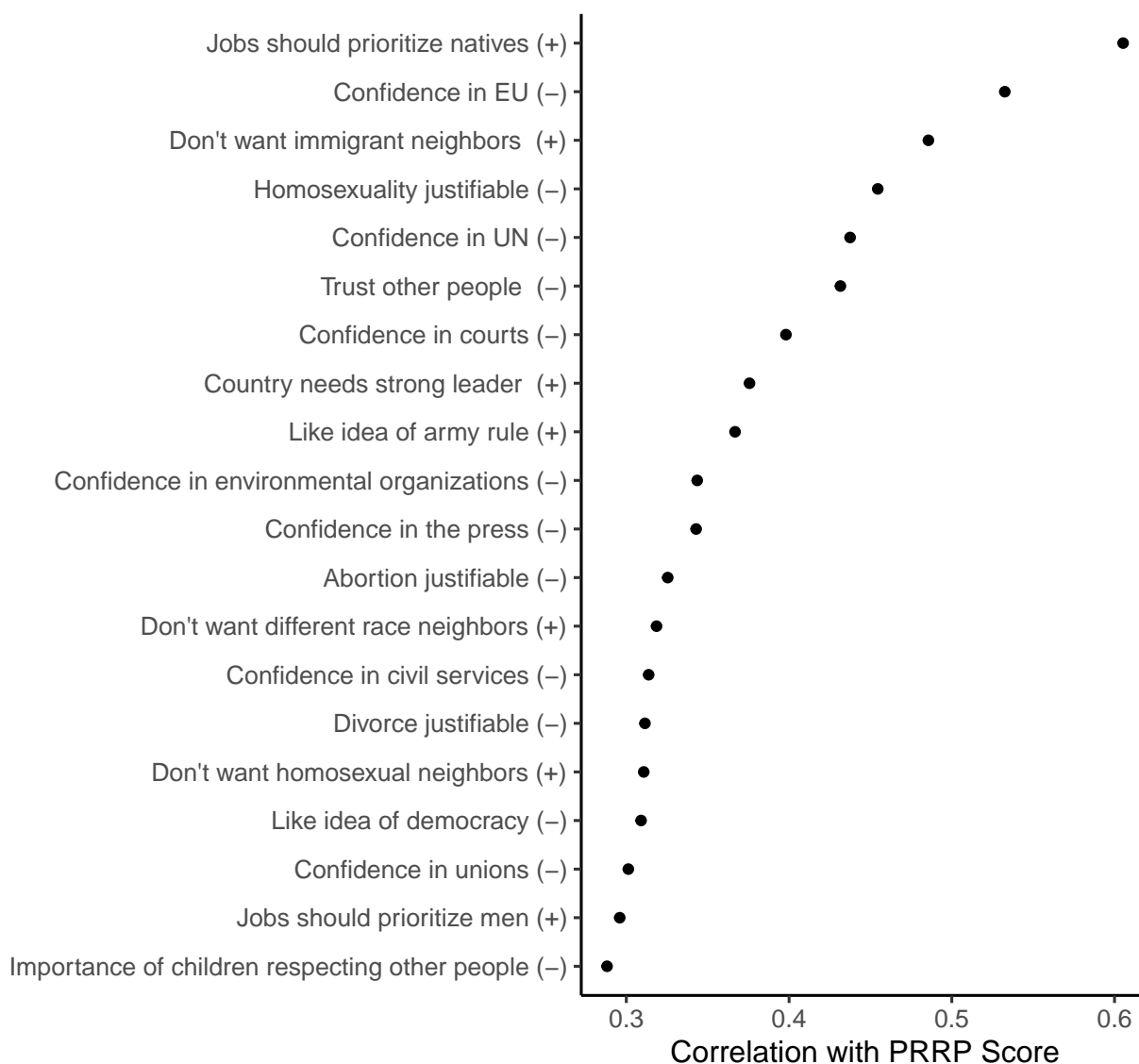
Figure A.4: Covariates Most Strongly Correlated with the PRRP Score
