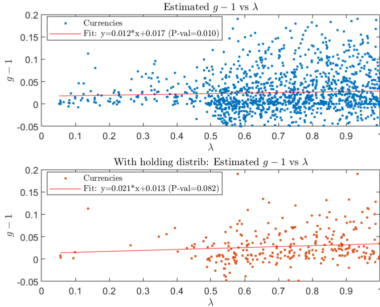
Figure 6: Correlation between long-run money growth g and convergence speed \lambda . Notes: We scatter-plot estimated g and \lambda for all tokens with g \in (0.95, 1.2) and \lambda \in (0, 1] in the full sample (upper panel) and the subsample with holding distribution data in 2023 (lower panel). Red line represents the linear fit of the relationship between g and \lambda .
