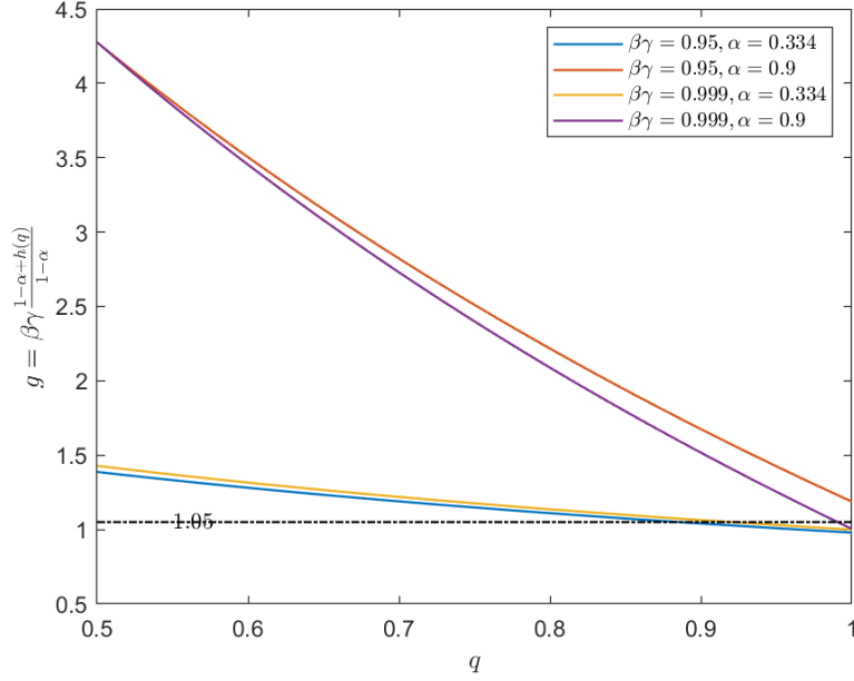
Figure 3: Back-of-envelope calculation of commitment probability q in the baseline setup. Notes: We compute the steady-state money growth rate in the baseline setup with probabilistic commitment, i.e., Proposition 8: g = \gamma\beta \frac{1-\alpha+h(q)}{1-\alpha} with h(q) = \frac{(1-\gamma\beta q)(\alpha+1)}{2\gamma\beta q + \alpha + 1} , with \gamma\beta \in \{0.95, 0.999\} and \alpha \in \{0.334, 0.9\} .
