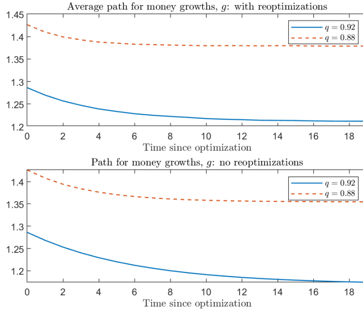
Figure 5: Simulated paths for money growth rates. Notes: We fix \beta = 0.95, \gamma = 1.05, \alpha = 0.85, \zeta = 90, \eta = 0.01 and solve the model with q = 0.92 and q = 0.88 . Starting from an optimization state, we simulate 3,000 tokens for 20 periods, and compute average money growth rates across firms. The upper panel allows reoptimization shocks whereas the lower panel does not.
