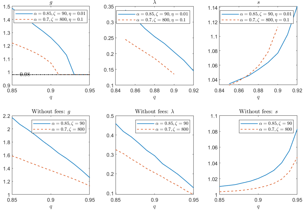
Figure 4: Optimal monetary policies and commitment probability q . Notes: We fix \beta = 0.95 and \gamma = 1.05 . The upper (lower) panel presents our model with (without) fees and endogenous velocity. We solve the model by setting the lower bound for g to 0.98. For figures of optimal \lambda and s in the upper panel, we plot the region where the corresponding optimal g does not hit the lower bound.
