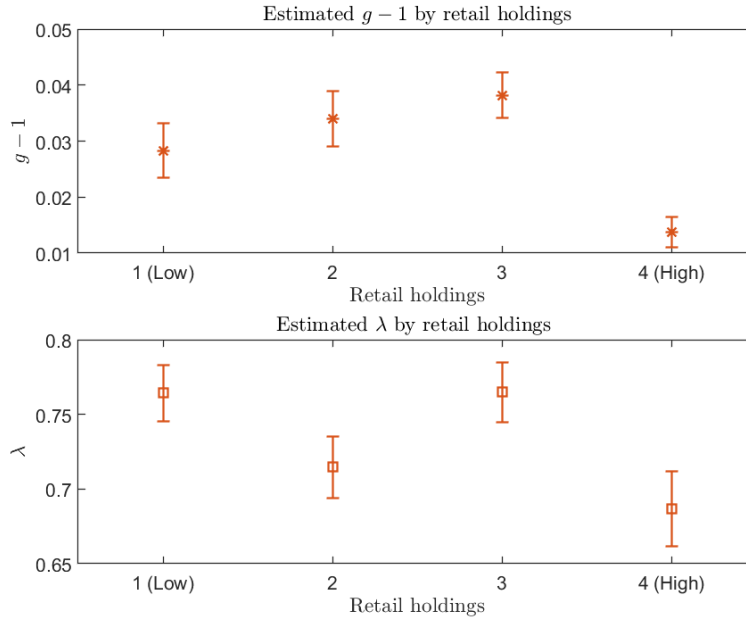
Figure 8: Retail holdings and monetary policy: portfolio sorts. Notes: We sort tokens with g \in (0.95, 1.2) and \lambda \in (0, 1] by their levels of retail holding into 4 equal groups and plot the mean (* and \square ) and the standard error of means (error bars) of g and \lambda for each group.
