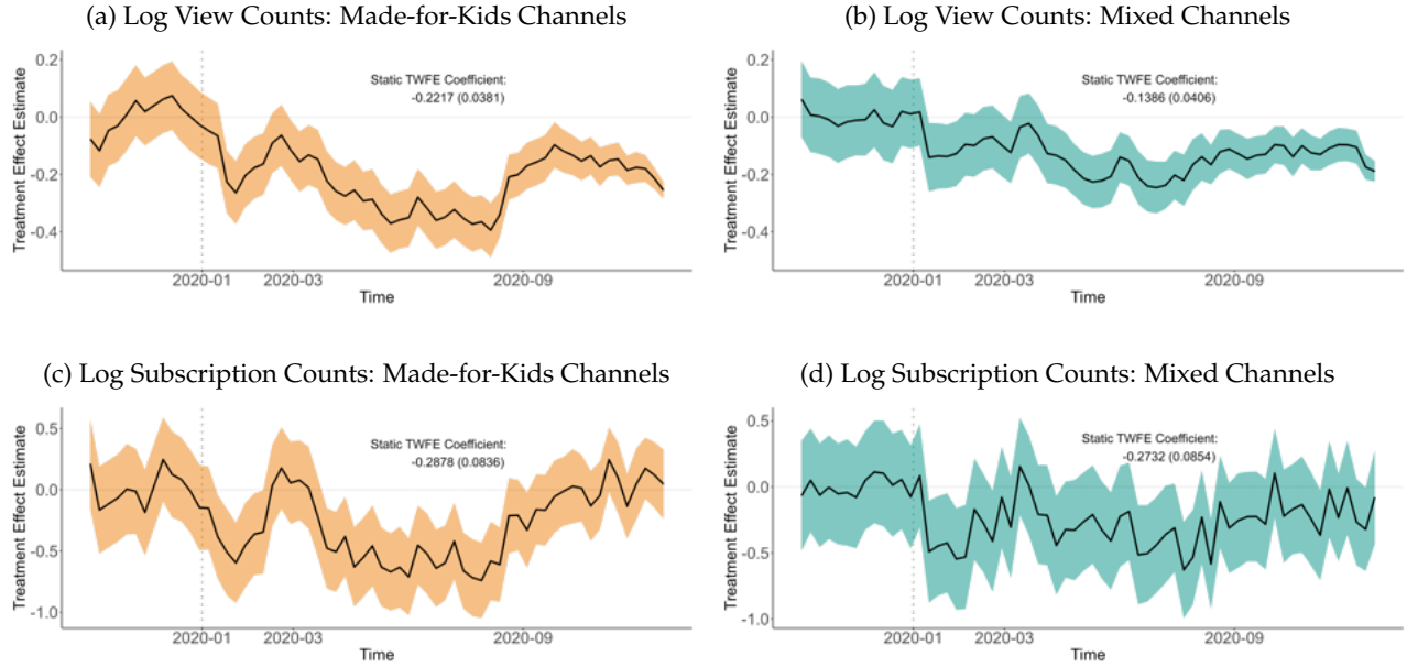
Figure 8: Time-Varying Treatment Effects on Demand-Side Outcomes
