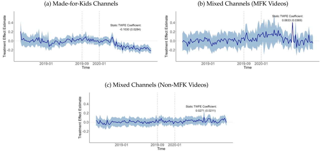
Figure C.3: Time-Varying Treatment Effect on Like/View Ratio
