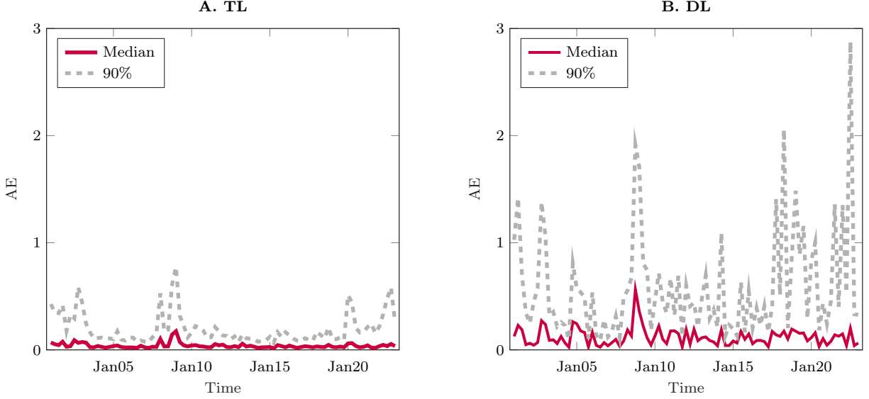
Figure 3: Outliers for TL vs. DL. In this figure, we compare the 90th percentiles of out-of-sample pricing errors (absolute errors in BSIV) for the TL and DL model.
