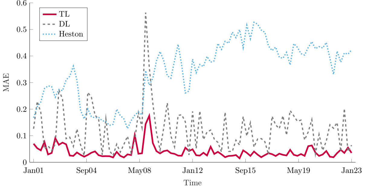
Figure 2: Out-of-sample pricing errors. This figure reports the out-of-sample median-absolute pricing errors (in terms of BSIV) for TL, DL, and the Heston model at quarterly frequency from 2001Q1 to 2023Q1. At the end of each quarter, the models are trained using data from the past 3 months, and the pricing errors are computed using data in the following 3 months.
