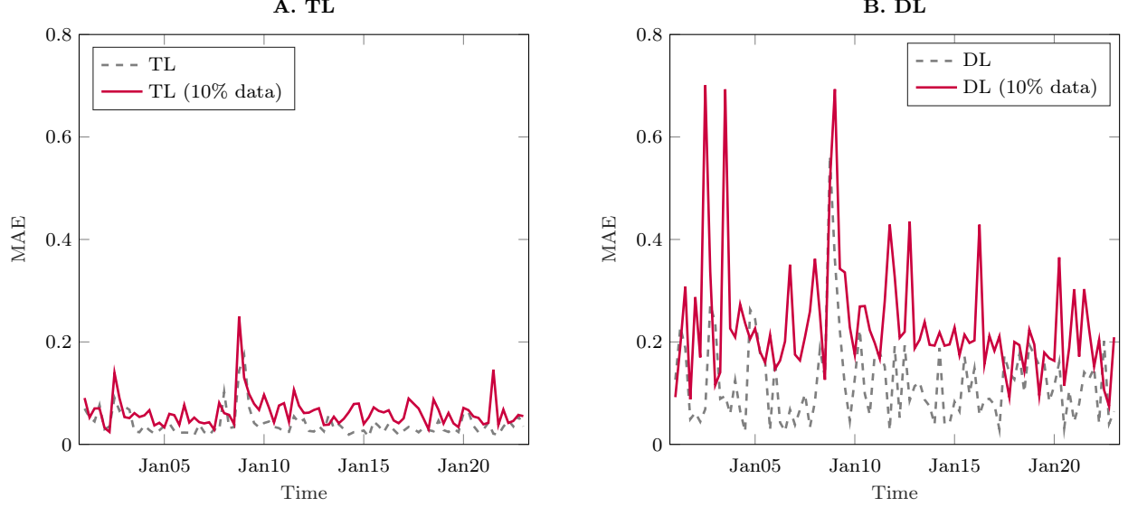
Figure 4: TL vs. DL with small training sample. In this figure, we compare the out-of-sample BSIV-MAE for TL against those of DL when the training sample is reduced to 10% of the original size.
