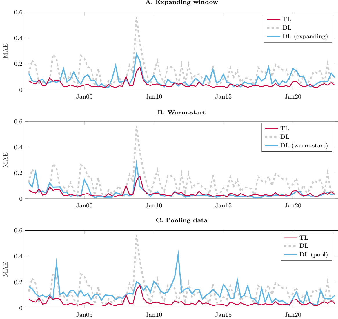
Figure 7: TL vs. DL under expanding windows and warm-starting. This figure compares the out-of-sample median-absolute pricing errors for TL and DL under the rolling-window setting against those of two differently-trained DLs. The expanding-window approach retraines the DL in each quarter using all the data available up to that quarter, with network parameters initialized randomly each time. The warm-starting approach follows the rolling-window procedure but trains the DL in each quarter by initializing its parameters using the values from the model trained in the previous quarter.
