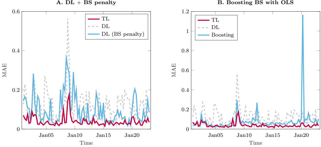
Figure 11: Comparison with alternative ways to incorporate structural model information. In this figure, we compare the out-of-sample BSIV-MAE for TL against those of DL that treats the Black-Scholes model restrictions as constraints (Panel A) and a Black-Scholes boosting model (Panel B).
