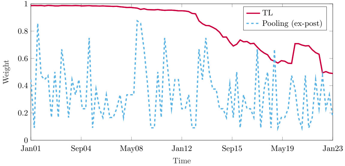
Figure 14: Weights of Synthetic Data. The figure illustrates the weights of synthetic data in transfer learning and the optimal weights derived using a deep learning-based Bayesian method. At each time point, we extract the weights corresponding to the minimum value from multiple sets of weights to determine the optimal weights.
