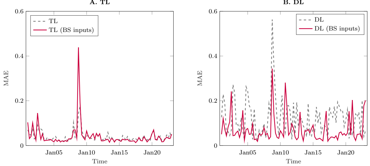
Figure 8: TL and DL with model-implied inputs. TL (BS inputs) refers to that within the transfer learning framework, we retain solely the inputs utilized in the Black-Scholes model. Similarly, DL (BS inputs) means that within the deep learning framework, we retain solely the inputs utilized in the Black-Scholes model.
