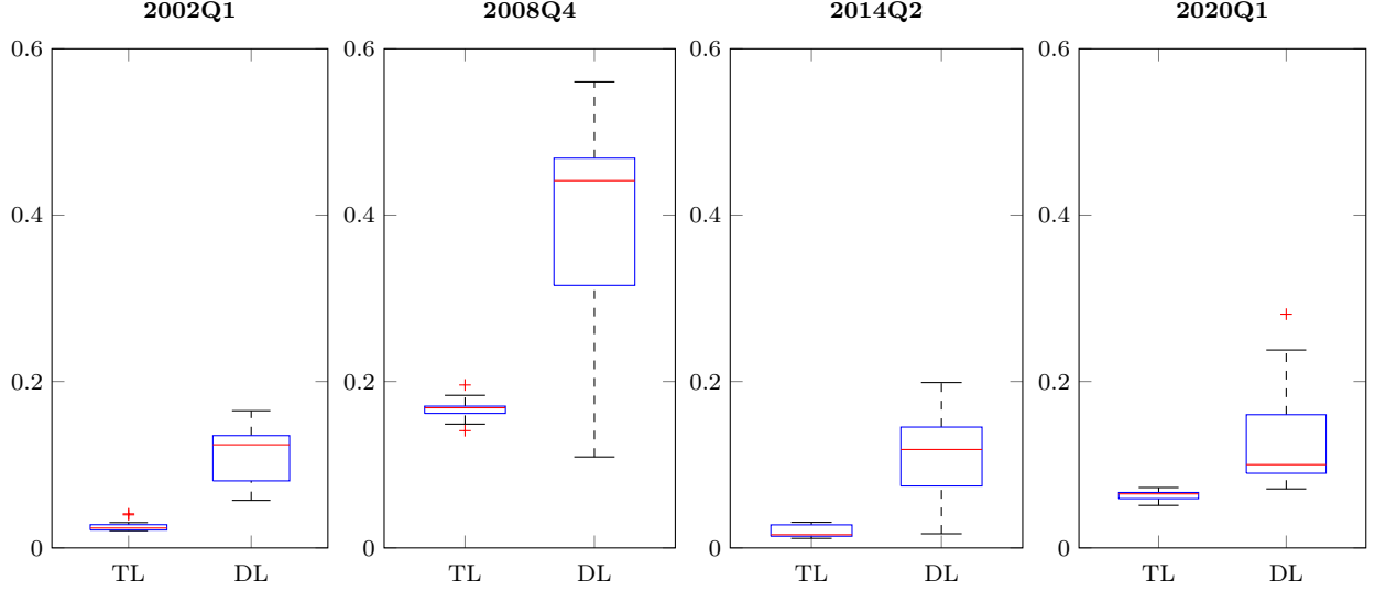
Figure 5: Stability of TL vs. DL. In this figure, we examine the distribution of out-of-sample BSIV-MAE for TL and DL at four points in time as the random seeds for network training change.
