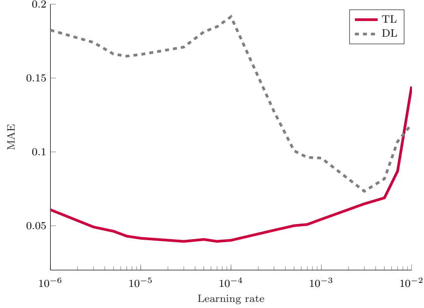
Figure 10: Optimal Learning Rate in Target Domain. The figure demonstrates the relationship between the learning rate and the out-of-sample pricing errors. We retrain the TL and DL model under different learning rates. The out-of-sample pricing errors (BSIV-MAE) are then averaged over the full sample.
