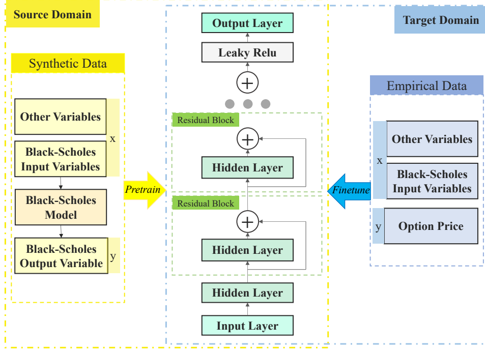
Figure 1: The Transfer Learning Framework. This figure illustrates the application of our adopted transfer learning framework in the context of option pricing.
