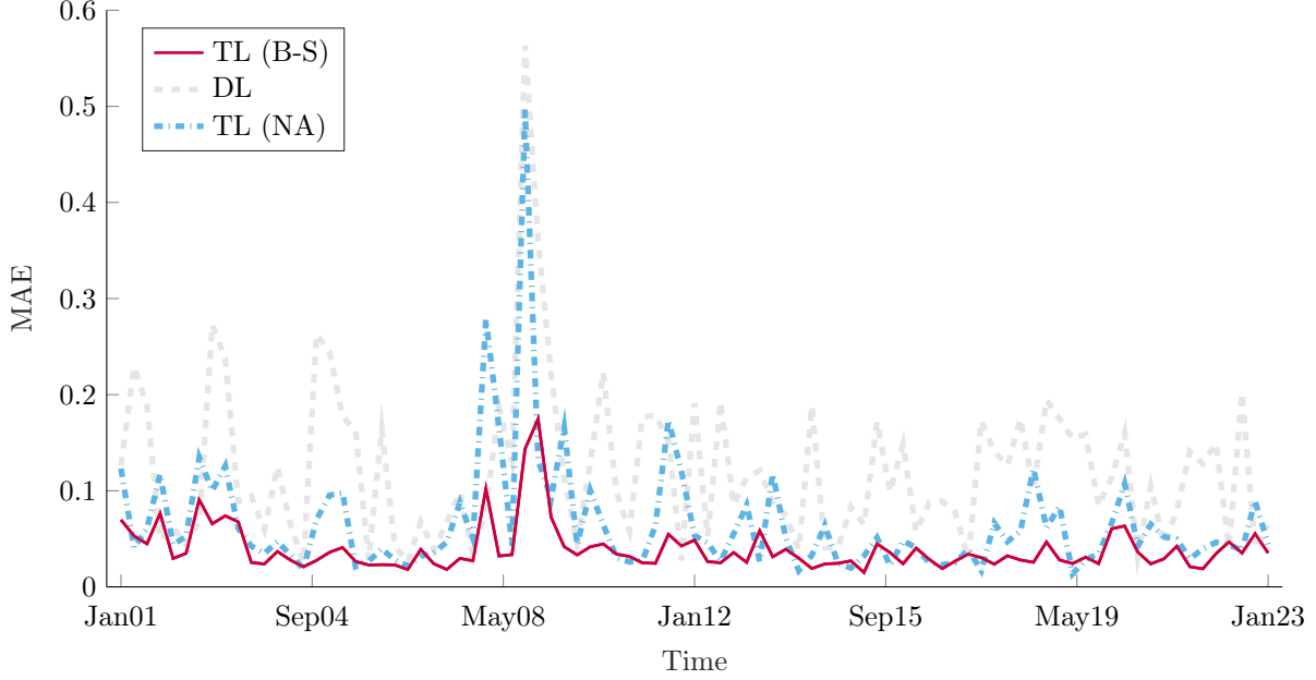
Figure 9: TL with strong vs. weak structural restrictions. In this figure, we compare the out-of-sample median-absolute pricing errors for TL that uses the Black-Scholes model in the source domain against another TL that imposes only the model-free no-arbitrage restrictions in the source domain. Specifically, the synthetic put option prices are randomly drawn from between the lower and upper bounds under the no-arbitrage conditions ( \max(Ke^{-rT} - S, 0) and Ke^{-rT} ).
