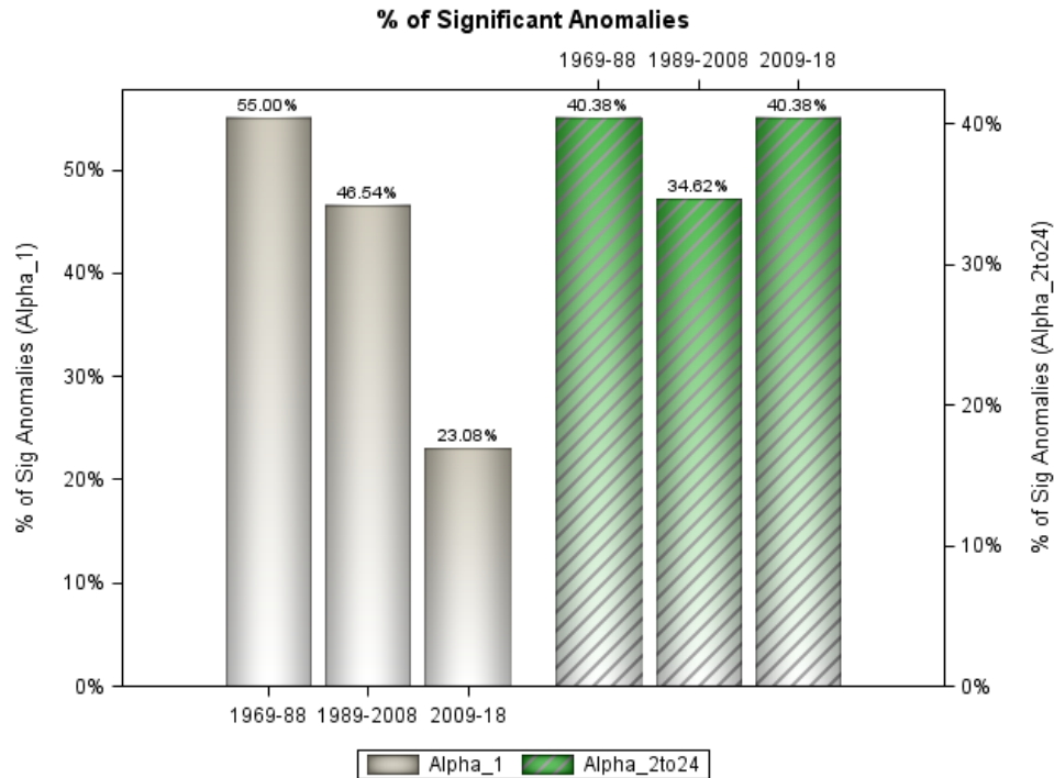
Panel A: Short and Long-term Percentage of Significant Anomalies
