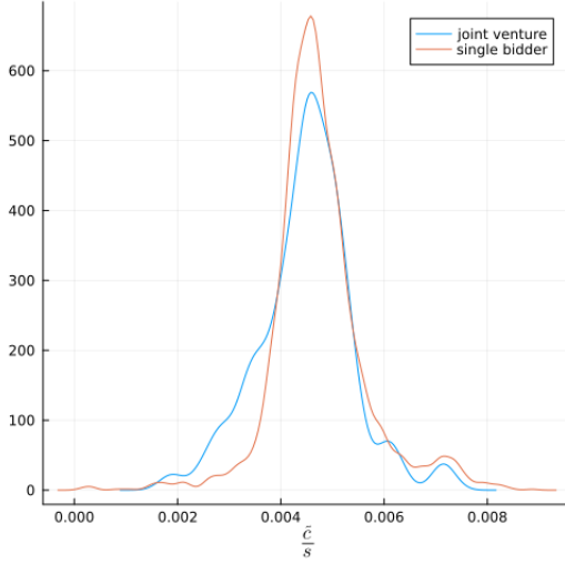
(a) A Homoskedasticity Case
