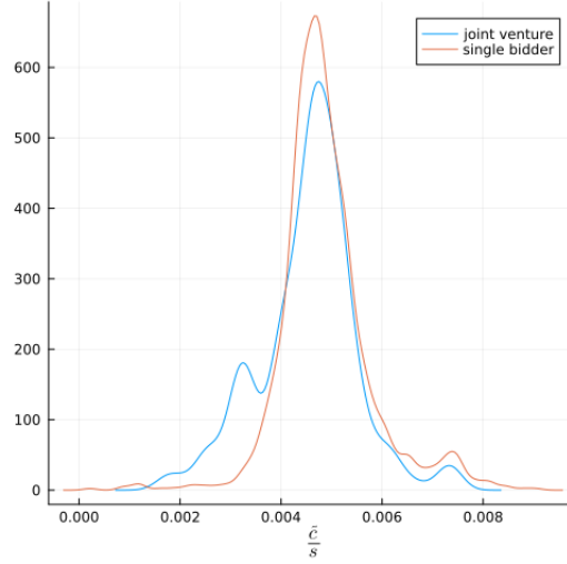
(b) A Heteroskedastic Case
