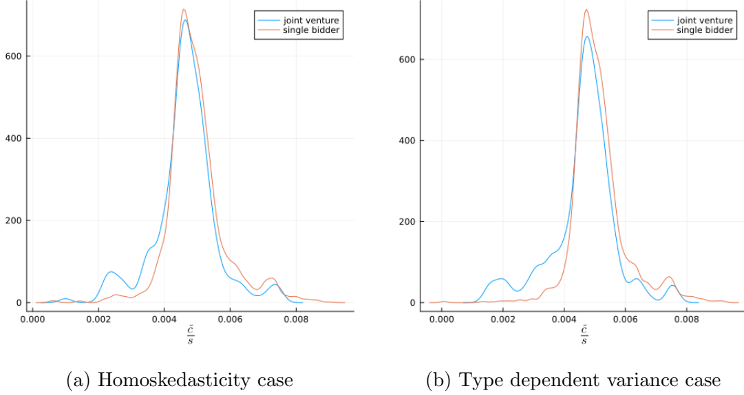
Figure A3. Density estimations of \frac{\tilde{c}_i}{s_i} . We focus on the entrants in the auctions in which at least one joint venture participate. Blue line represents the density for joint venture and red line represents the density for single bidder. Panel (a) is the result when we assume homoskedastic variances. Panel (b) is the result when we use type-dependent variance estimations.
