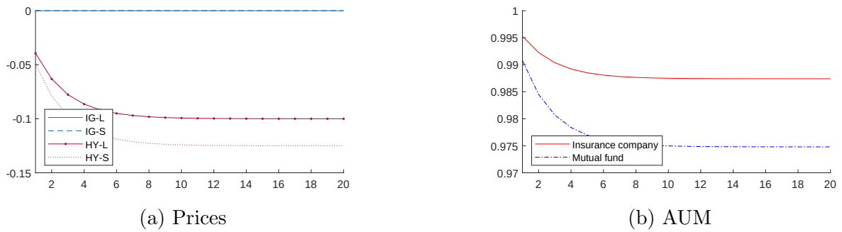
Figure 2: Beta equals 0
