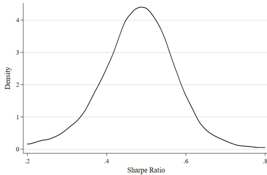
Figure A7: Portfolio Sharpe Ratios
