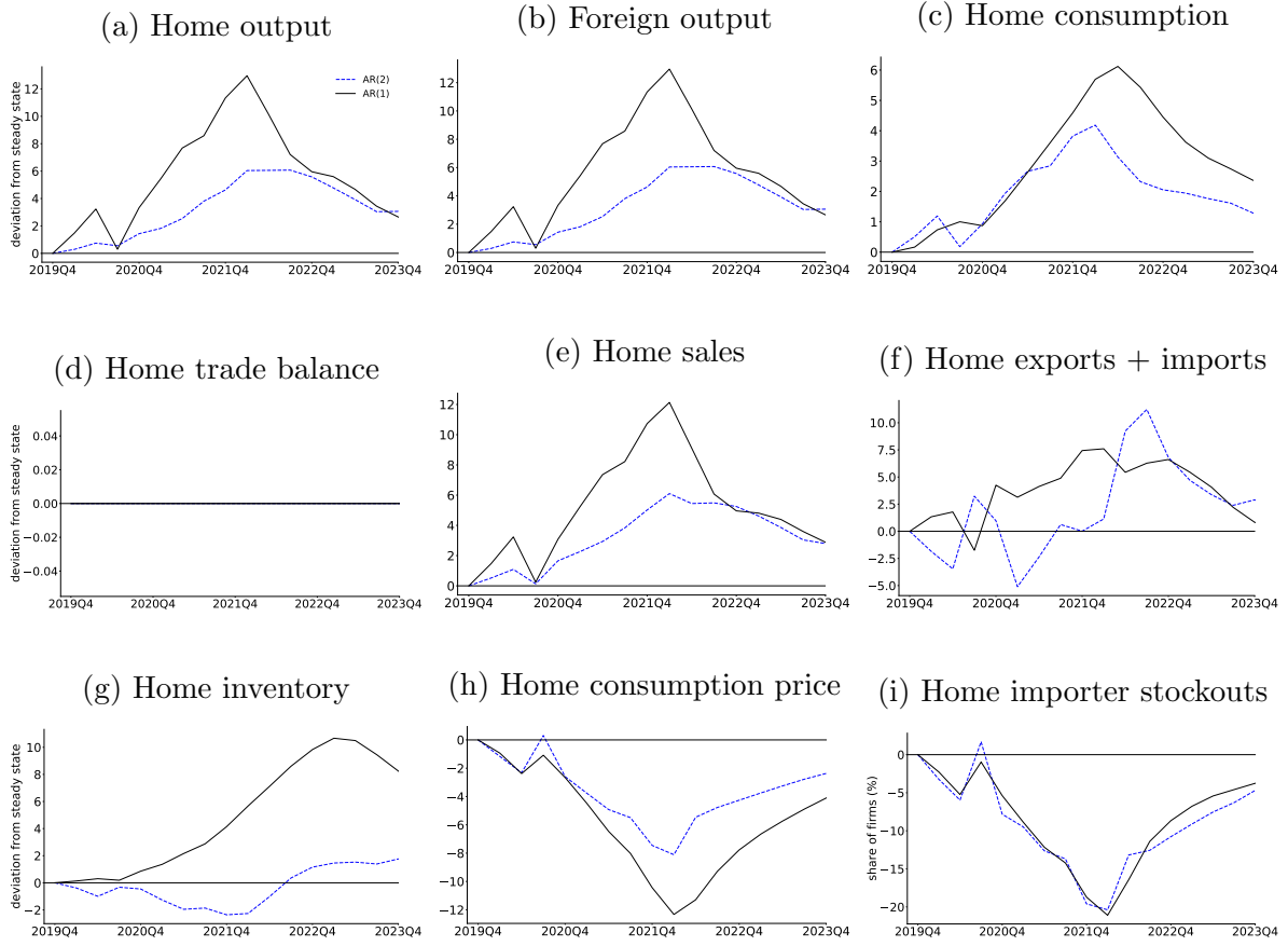
Figure 20: The effect of import delays: AR(1) v AR(2)
