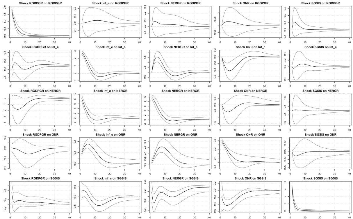
Figure 2: BVAR IRFs
