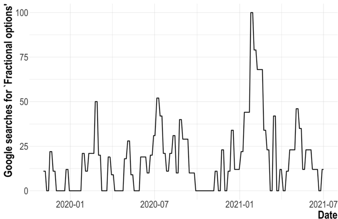
Figure A5: Google searches for fractional options
