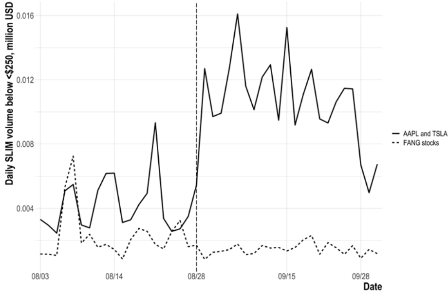
Figure A6: SLIM trading volume around stock splits
