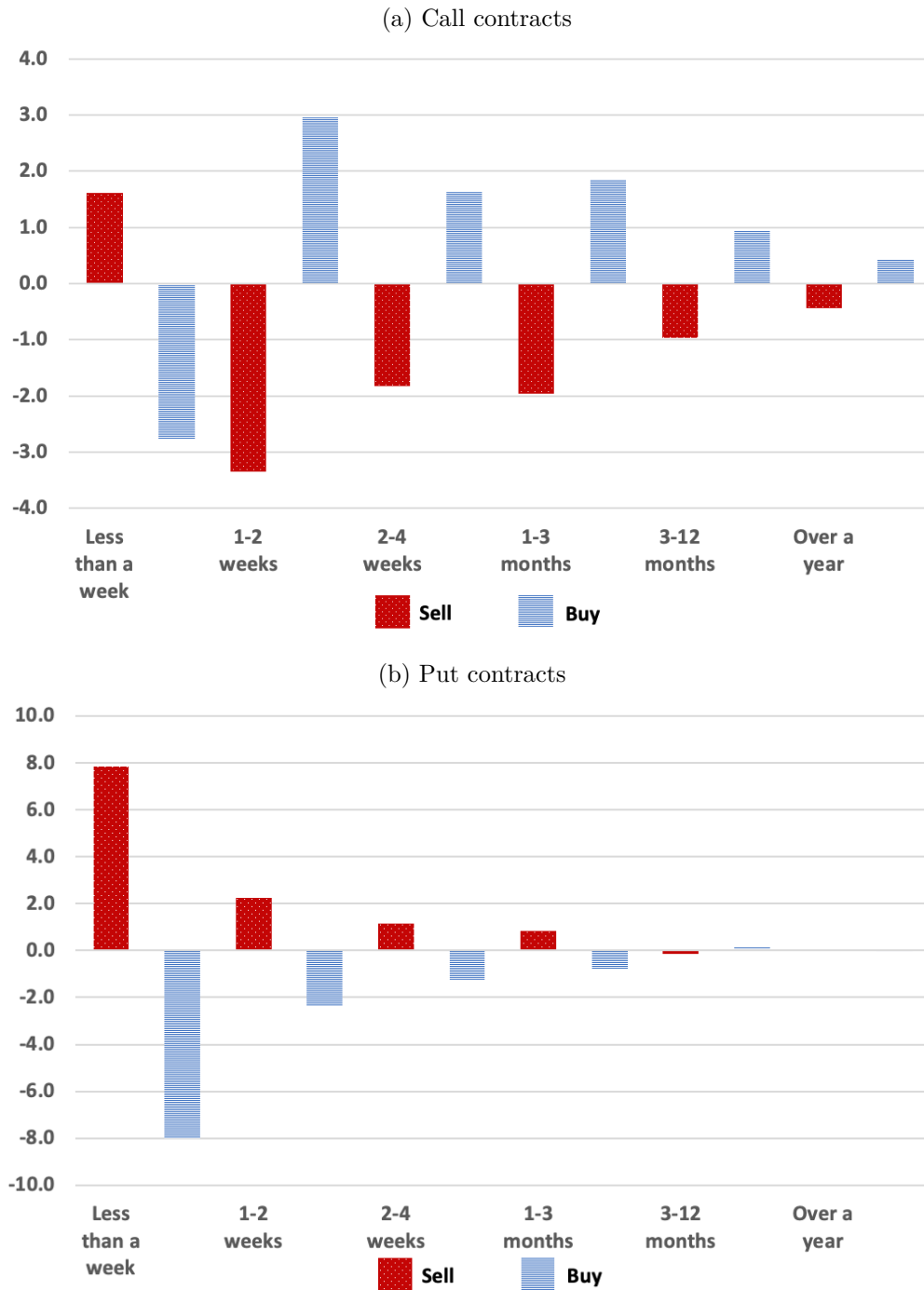
Figure A3: SLIM performance by contract type, trade direction, and time to expiration
