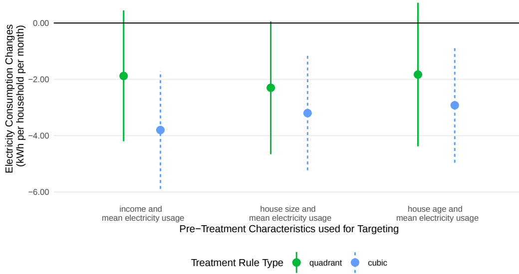
Figure 3: Estimates of the energy savings from targeted treatment assignment
