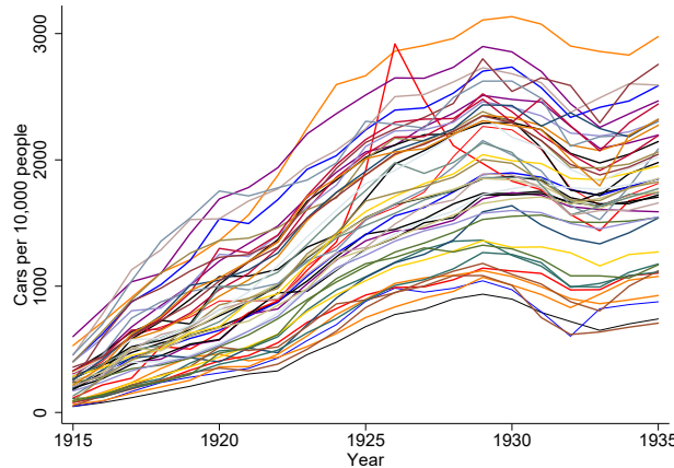
Figure 1 – State diffusion curves
