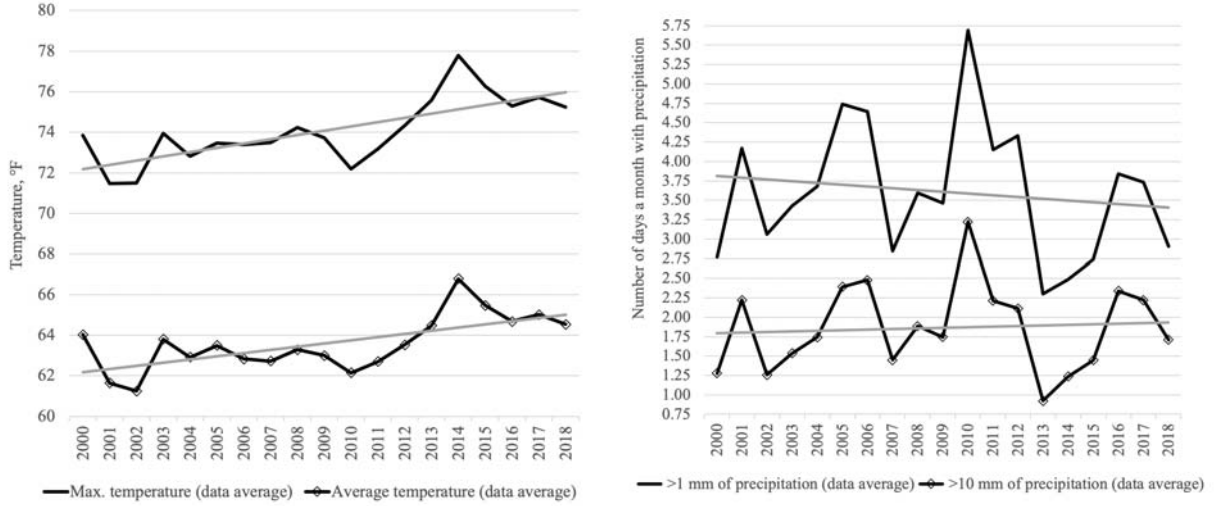
Figure 6: Weather data over the period of analysis. This figure shows the dynamics of the monthly mean of four weather-related variables in all the U.S census tracts in California. Panel A displays the mean of the maximum temperature of the month and the mean of the average temperature of the month. Panel B displays the mean of the days with at least 1 mm. and 10 mm. of precipitation per month. Both panels show the average linear trend of these variables.
