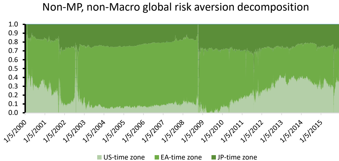
Figure 3: The time zone factor model: estimated global risk aversion decomposition, by time zones.
