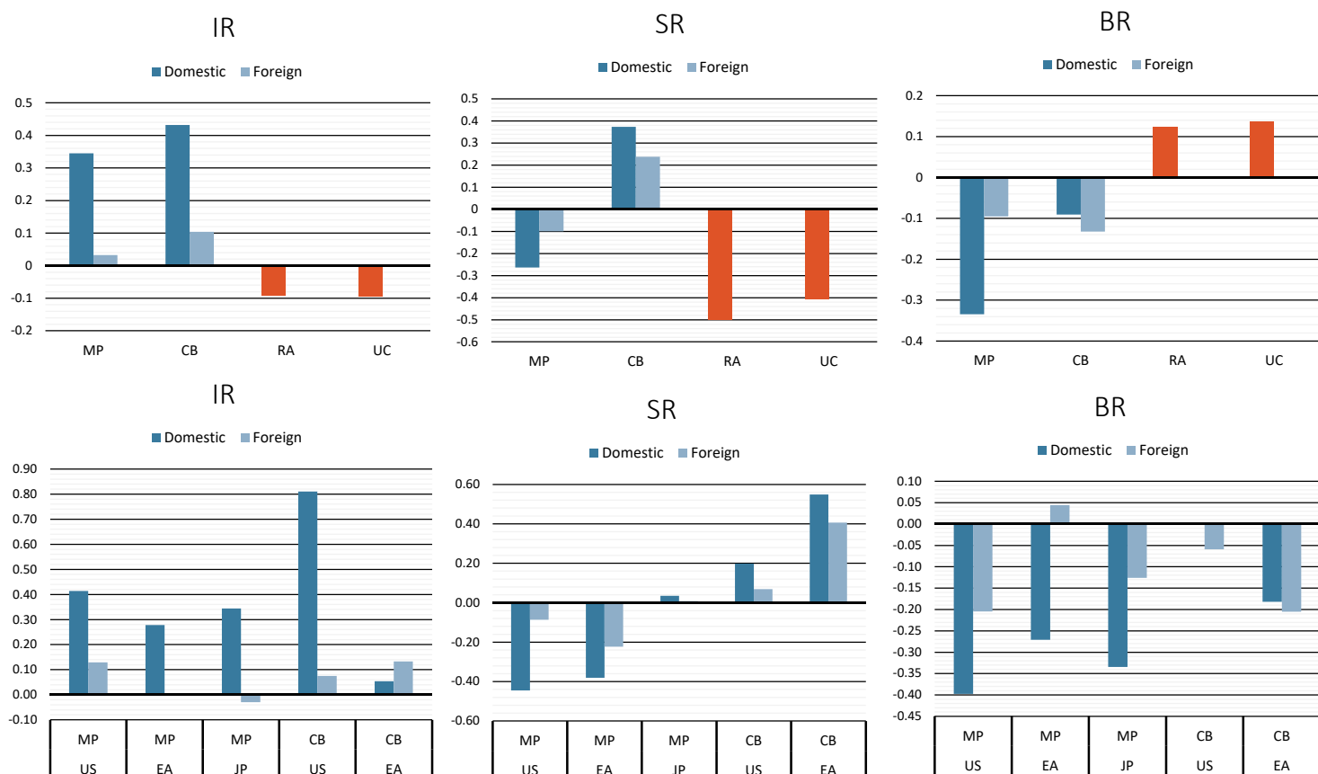
Figure 2: The effects of MP and risk shocks on interest rates (IR), stock returns (SR) and bond returns (BR).
