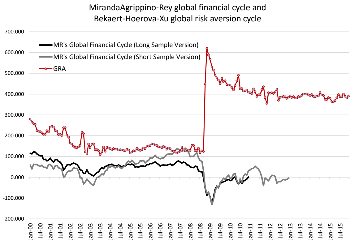
Figure 4: Comparisons to Miranda-Agrippino and Rey (forthcoming)'s global financial cycle variables.
