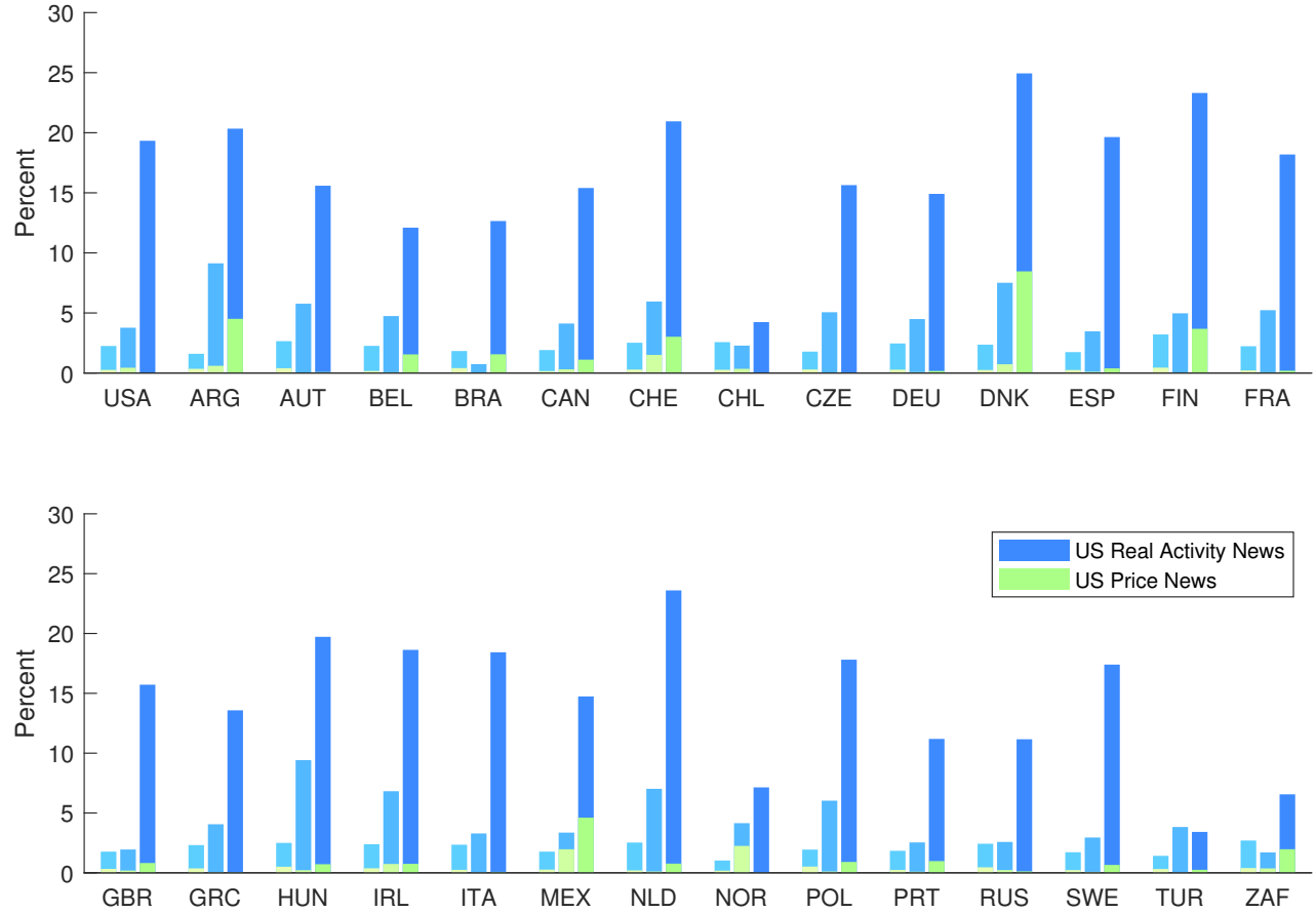
Figure C4: Daily, Monthly, and Quarterly R-Squared for Stock Indexes
