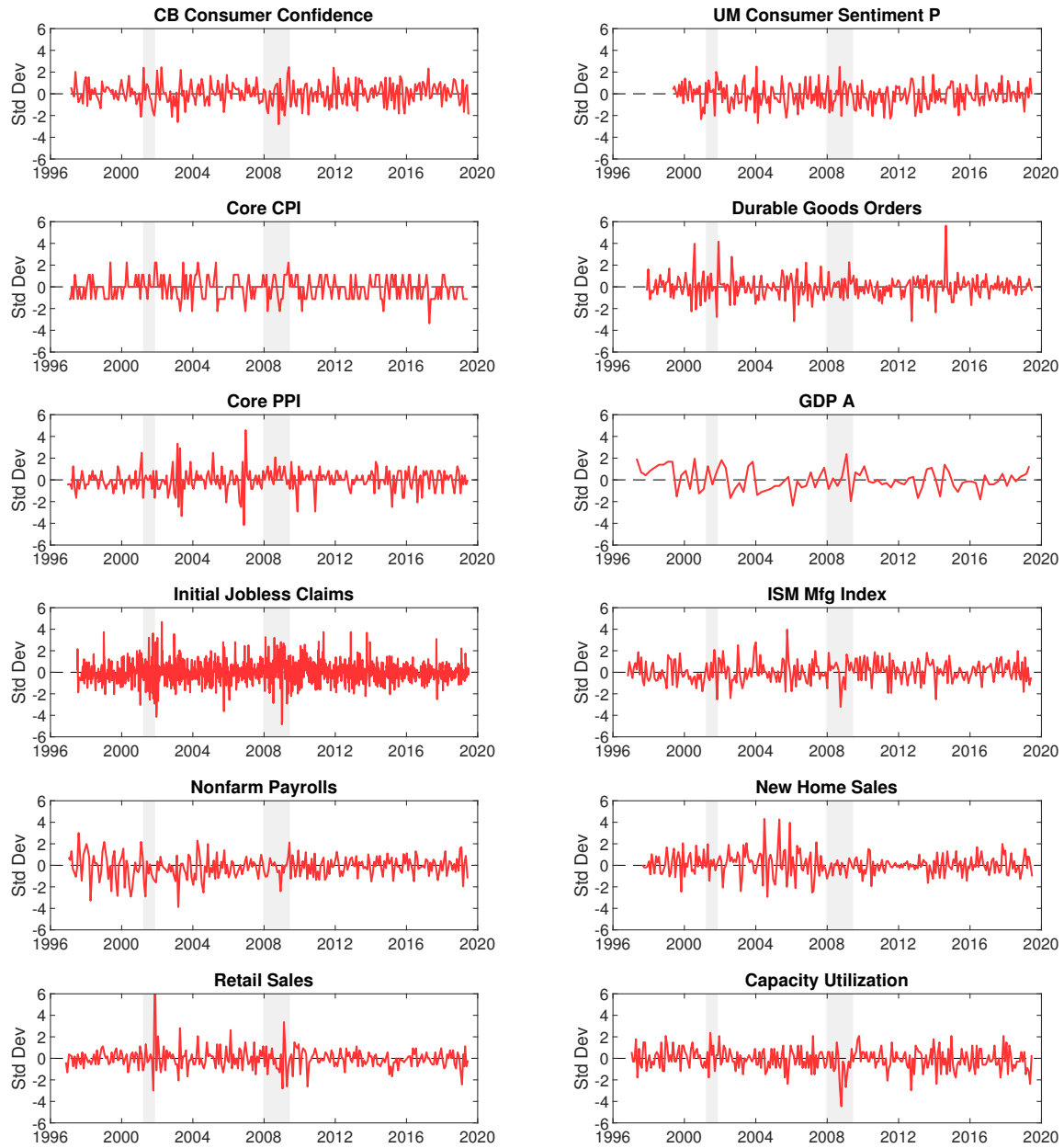
Figure B1: Time Series of Standardized Surprises
