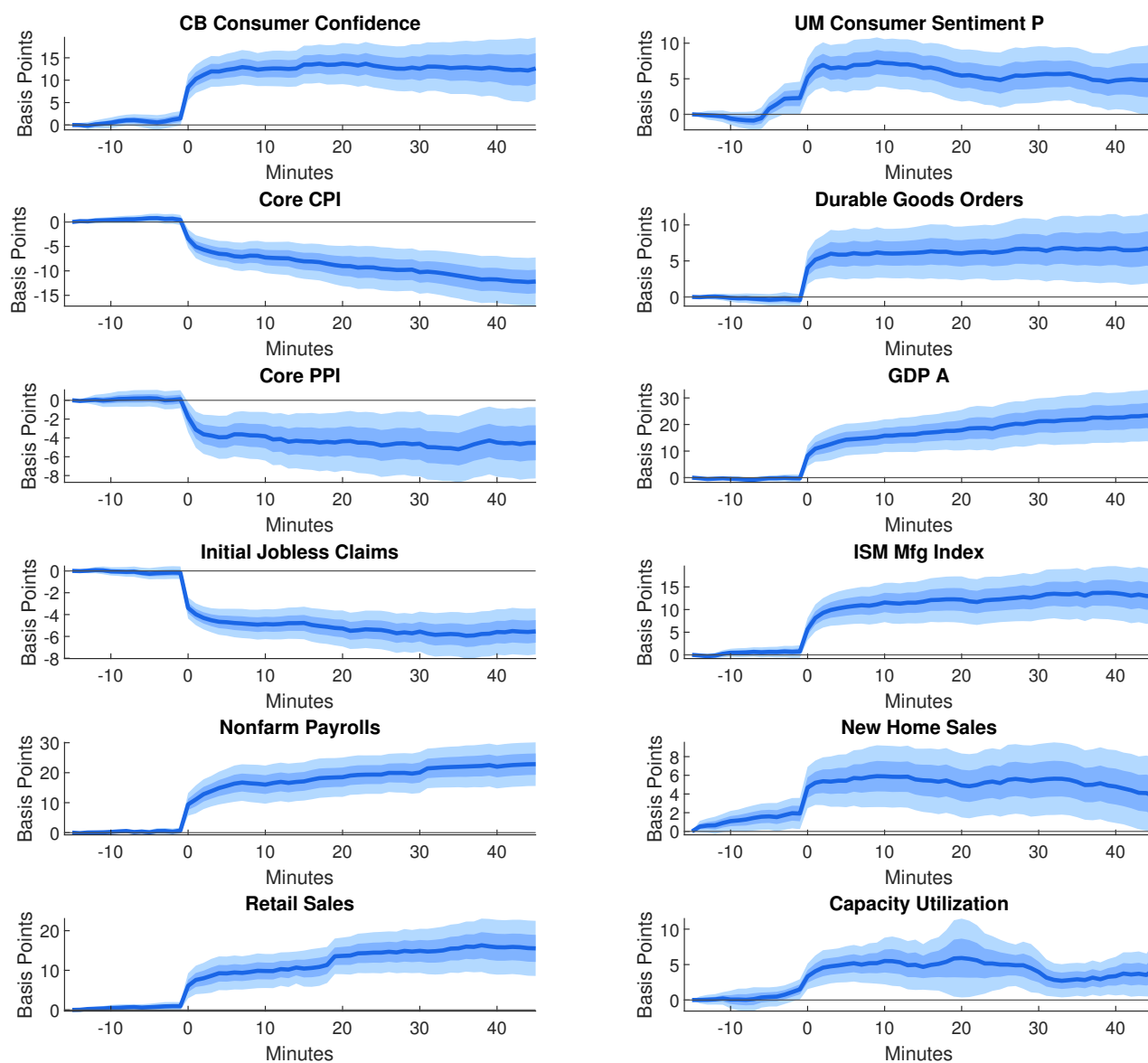
Figure C1: Average Paths within 60-minute Window for Selected Announcements
