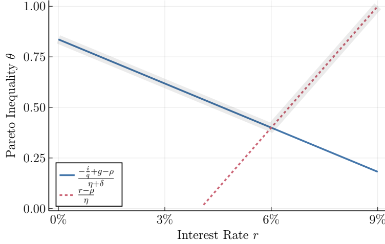
Figure 2: Pareto inequality \theta as a function of the interest rate.
