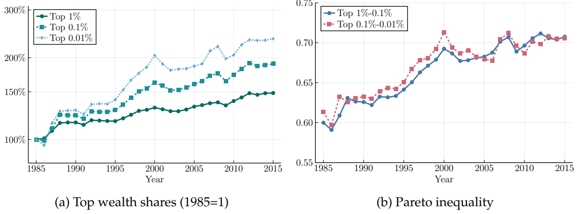
Figure 4: Rise in top wealth inequality (1985-2015)
