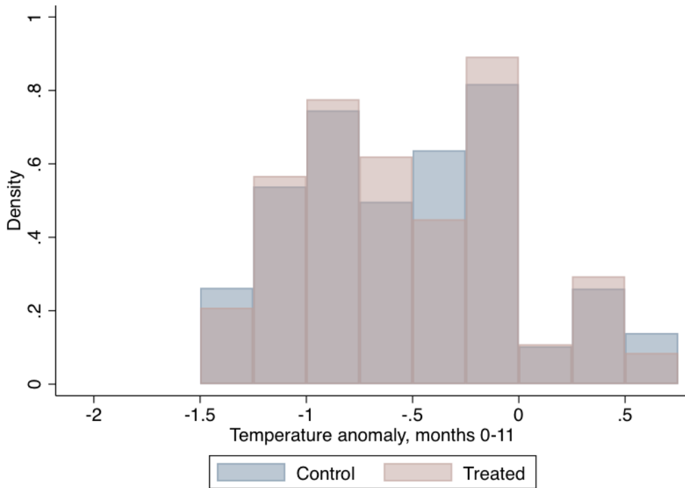
Figure 4: Distribution of Contemporaneous Temperature Z score
