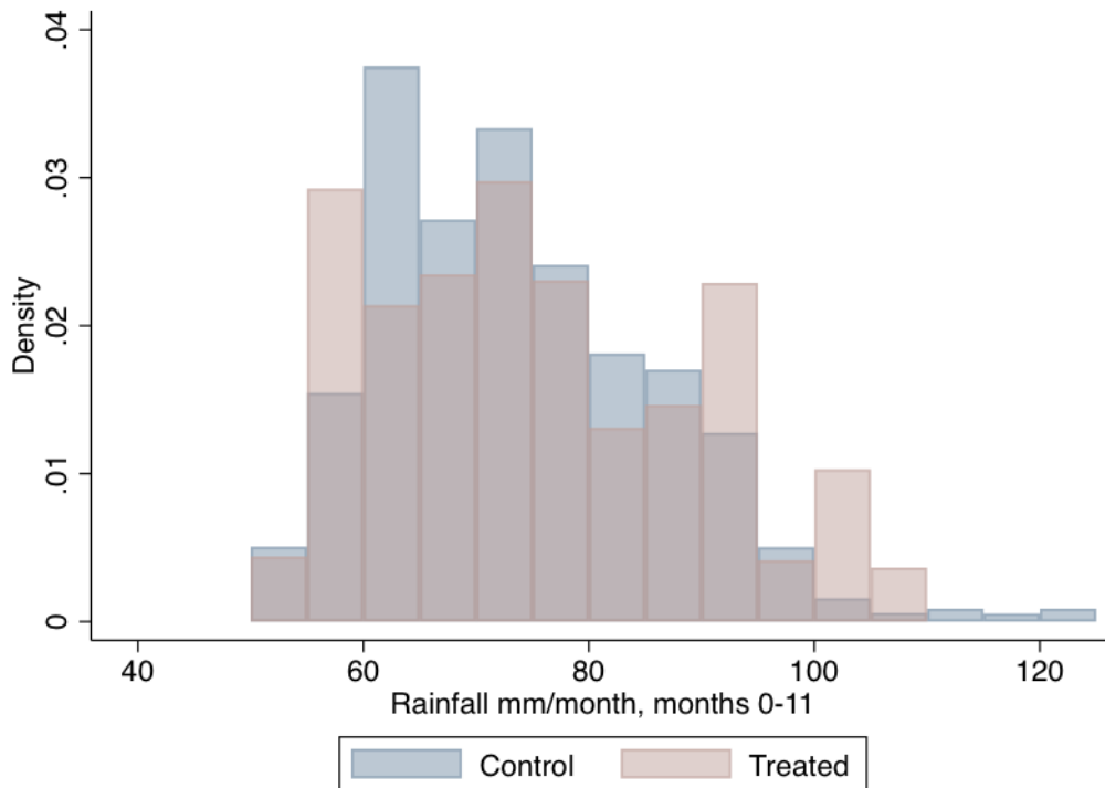
Figure 1: Distribution of Contemporaneous Rainfall
