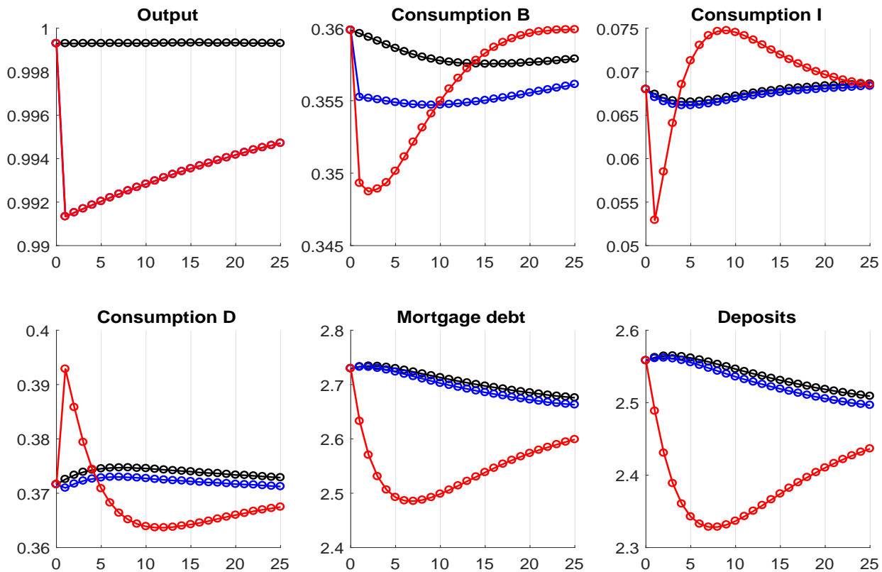
Blue line: non-financial recession, Red line: financial recession, Black line: no shocks.
