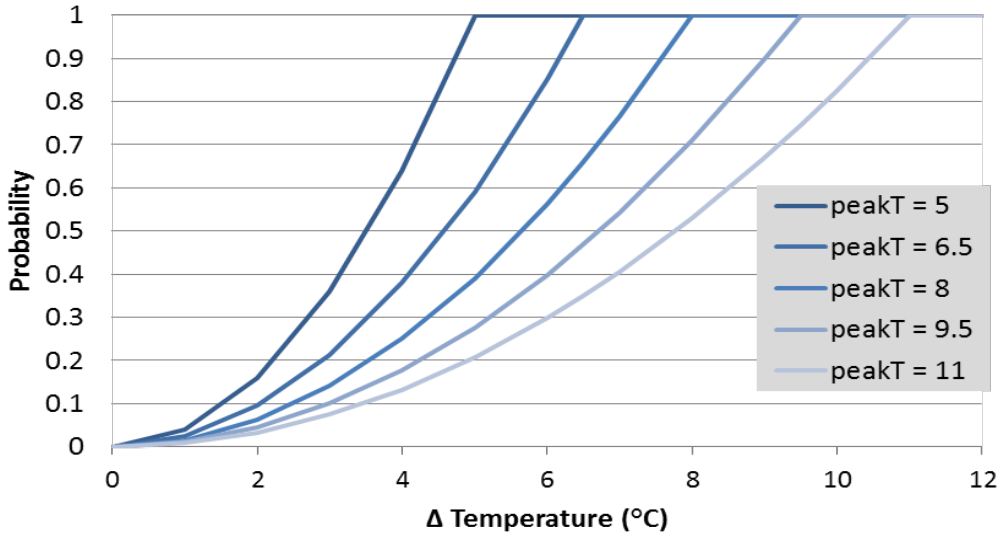
Figure 5—Probability of reaching a climatic tipping point as a function of peakT
