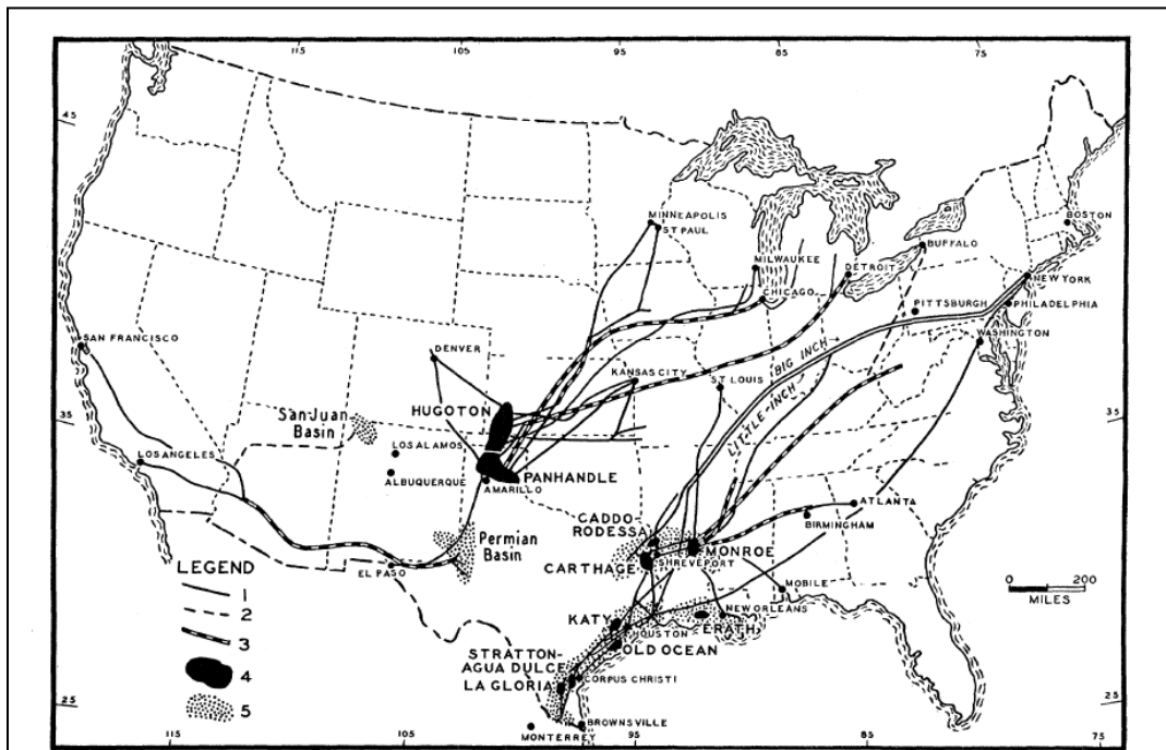
FIG. 1. Major interstate gas pipe lines in the United States, 1949. Legend: 1, pipe lines of 16-inch diameter or more originating in Mid-Continent and Gulf Coast areas; 2, pipe lines proposed or authorized; 3, double pipe lines; 4, principal gas fields; 5, other areas of scattered production supplying major interstate transmission lines.
